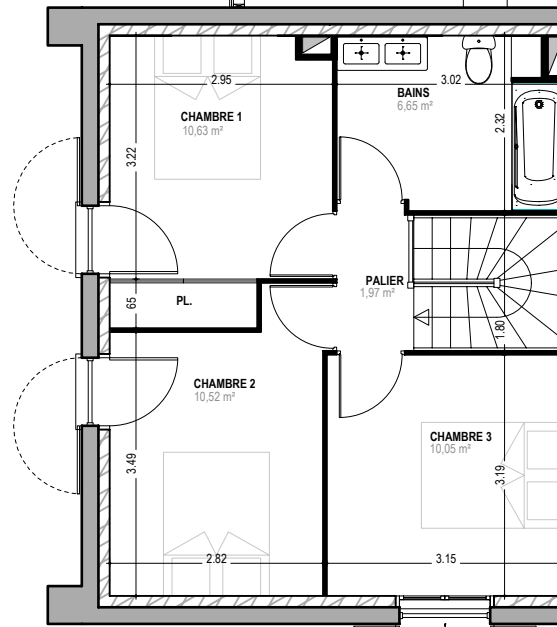
PLAN - R+1
