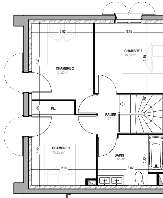
PLAN - R+1
